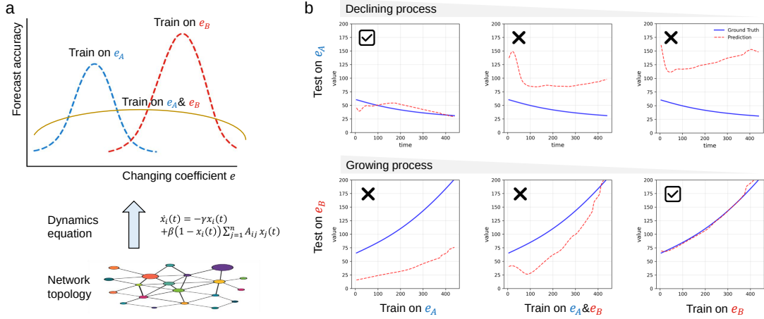
Figure 1: The generalization trap in network dynamics. (a) A generalist model trained on mixed data struggles to outperform specialized expert models. Network dynamics adopts the classic information dissemination model [40], in which the dynamic behavior is governed by the popularity coefficient. (b) Training and testing performance on cross-environment propagation dynamics, where e_A and e_B are propagation processes with different coefficients.
