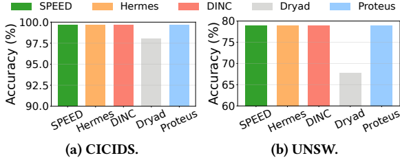
Figure 6: Accuracy under different datasets. We leave the full results in our appendix due to page limitations.
