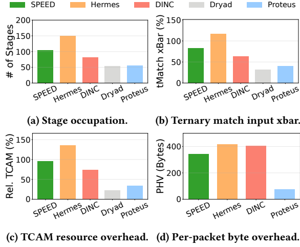
Figure 9: Switch resource consumption and inter-sub-tree coordination consumption under Fat-Tree topology.
