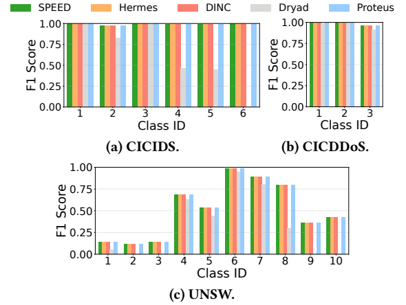
Figure 7: F1 score under different datasets.
