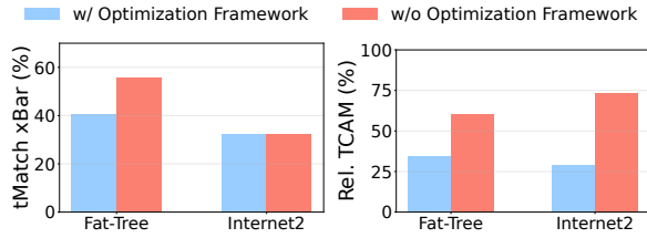
(a) Ternary match input xbar. (b) TCAM resource overhead.
