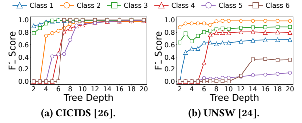
Figure 2: We train a 20-level decision tree for two typical intrusion detection datasets and measure the F1 score of six selected types when tree depth increases.
