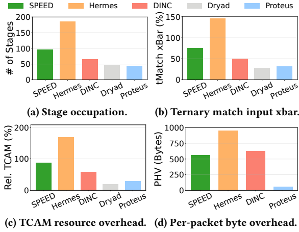
Figure 5: Switch resource consumption and inter-sub-tree coordination consumption under Internet2 topology.
