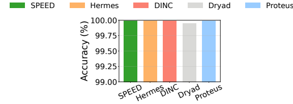
Figure 10: Accuracy under CICDDoS datasets.
