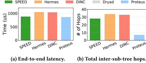
Figure 11: Detection speed under real-world DC topology, i.e., a Fat-Tree topology.
