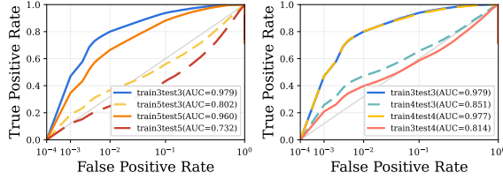
Figure 8: AUC curve of FORGE when the number of tabs differs between training and testing.
