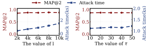
Figure 10: Parameter analysis of FORGE. We select the interval \tau and sequence length l .
