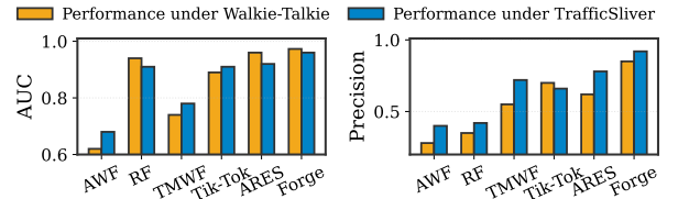
Figure 7: Comparison of AUC and precision under Walkie-Talkie and TrafficSliver on the single-tab setting.
