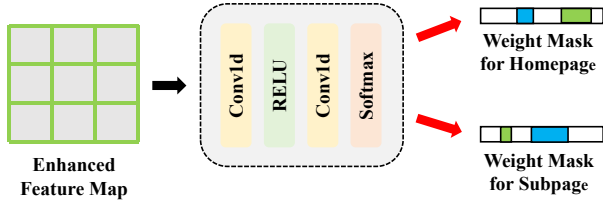
Figure 5: The architecture of Dual-Path Segmentation. A compact network derives two weight vectors from the features.
