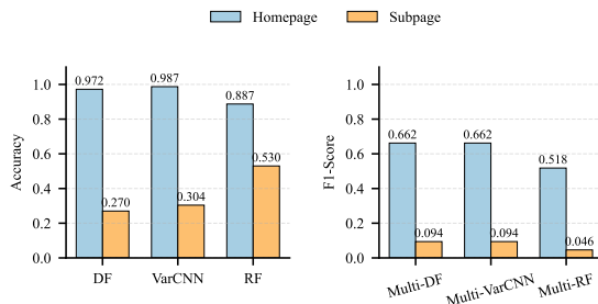
Figure 1: Comparison of WF Attacks on Homepage and Subpage for Accuracy in Single Table Scenario (Left) and F1-Score in Two Table Scenario (Right).
