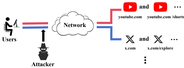
Figure 2: Threat Model of HiFi-WF.
