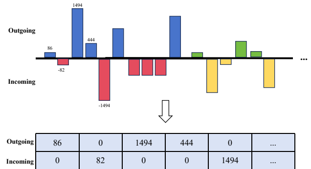
Figure 4: Traffic Sequences are Converted into a Dual-channel Input Matrix.
