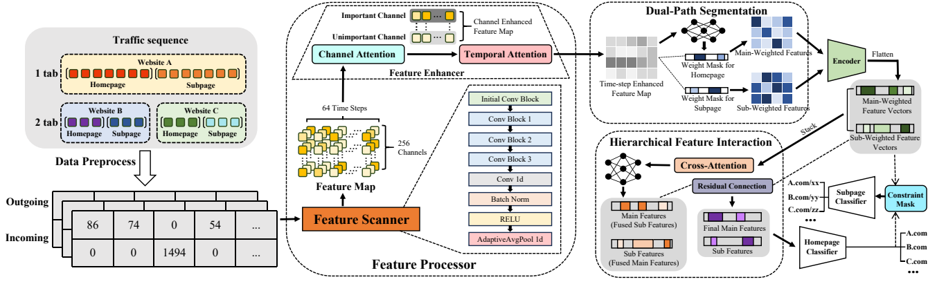
Figure 3: The overview of HiFi-WF.
