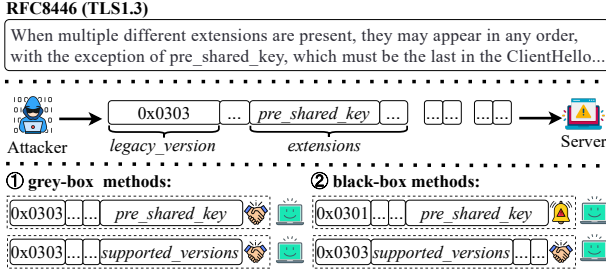
Figure 1: Limitation of existing methods
