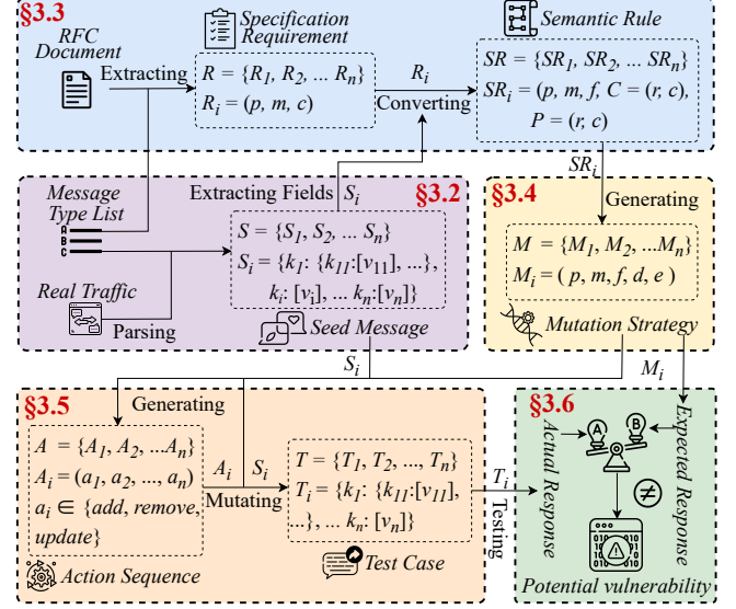
Figure 3: Overall architecture of SemFuzz
