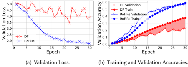
Figure 13: Comparison of DF and RoFiRE complexity when N = 90 and without augmentation.
