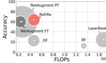
Figure 11: Comparison of RoFiRE and baseline models, in terms of FLOPs, parameters, and accuracy when N = 90 and T = 1000 .
