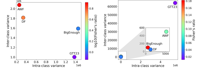
(a) Intra vs inter-class variance with log-scaled F-ratio using cell count. (b) Intra vs inter-class variance with F-ratio using circuit duration.
