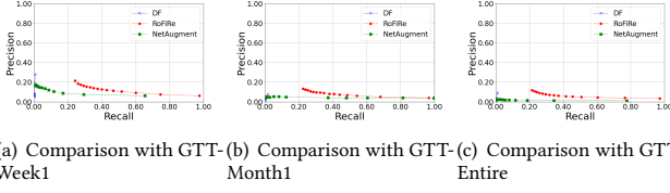
Figure 8: Real OW results of RoFiRE and baseline models across different unmonitored set sizes when N = 5 .
