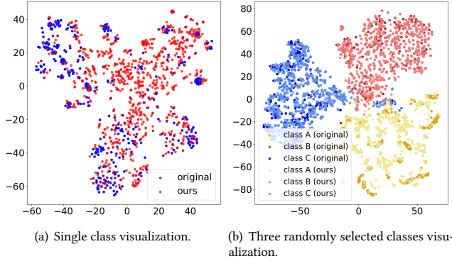
Figure 4: t-SNE visualization of 400 instances' embeddings from the penultimate FC layer, comparing the before (original) and after (ours) augmentation when \mathcal{N} = 10 and \mathcal{T} = 1000 .
