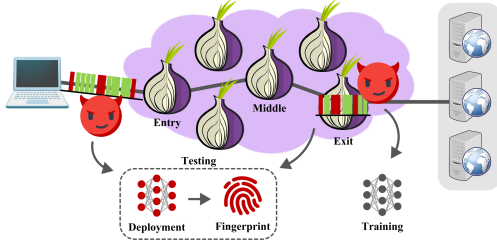
Figure 1: Threat model of a realistic WF adversary. The adversary collects training data from Tor exit relays and applies classifiers to infer website fingerprints.
