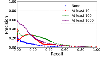
Figure 12: Real OW results of RoFiRE under varying trace-length filtering thresholds.
