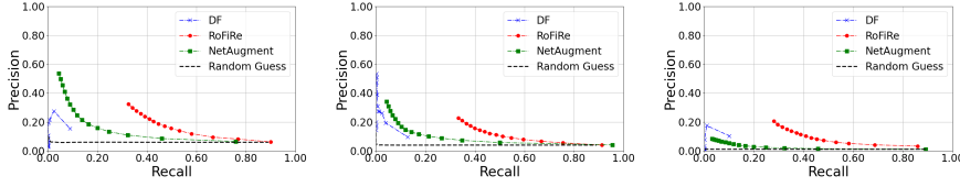
Figure 5: Real OW results of RoFiRE and baseline models across different unmonitored set sizes when N = 20 .
