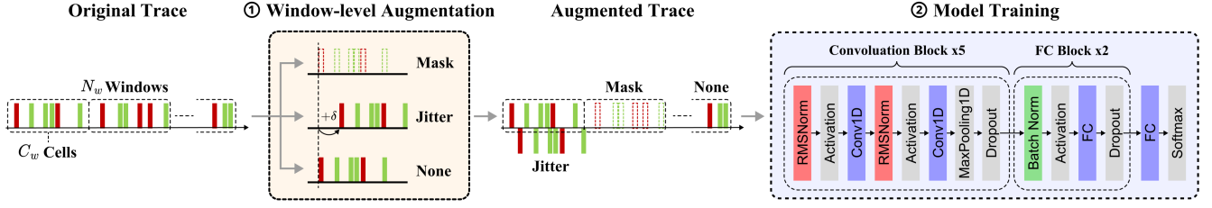
Figure 3: Overview of window-level augmentation and RoFiRe architecture.
