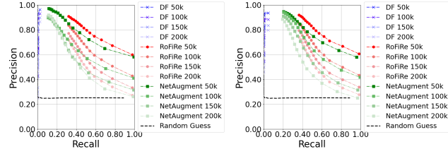
(a) Comparison of models with N = 10 . (b) Comparison of models with N = 20 .
