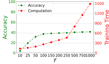
Figure 10: Accuracy and computational cost trade-off of augmentation in RoFiRE under varying T settings with N = 5 .
