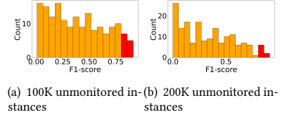
Figure 6: Per-class F1-scores ( N = 20 , T = 1000 , and \alpha = 0.2 ). Red bars denote highly fingerprintable classes.
