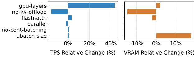
Figure 1: Single-parameter sensitivity of TPS and VRAM usage. Both versus the default value. Each bar shows the percent change from toggling one parameter while holding others fixed (positive = higher TPS / more VRAM).
