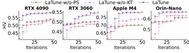
Figure 8: Ablation study on Parameter Selection (PS) and Knowledge Transfer (KT). Removing PS slows down improvement, while removing KT leads to a worse initial performance.
