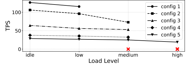
Figure 3: TPS of configurations across load levels. The x-axis lists load (idle to high); the y-axis is TPS. Each line is a configuration; red “x” marks configurations that failed.
