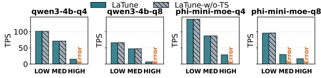
Figure 9: Ablation study of Two-Stage Optimization (TS) under varying system loads. “Error” denotes failures.
