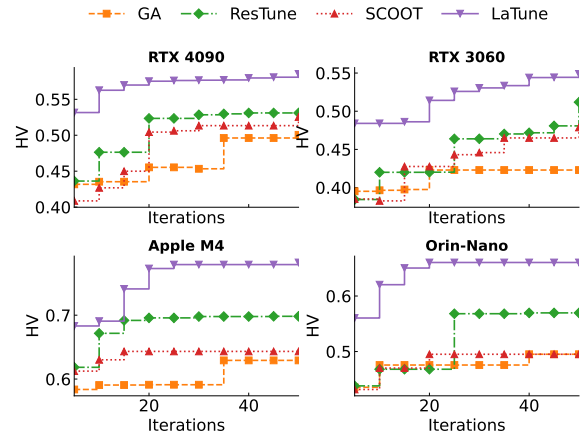
Figure 7: Tuning Efficiency Comparison. Curves plot the HV at each five iterations across methods on four devices. LaTUNE reaches higher HV sooner and achieves the best final HV across all platforms.
