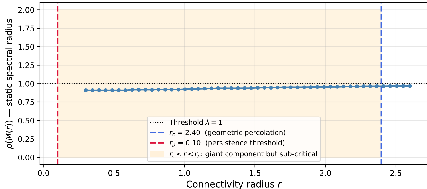
Static metapopulation capacity vs connectivity radius
