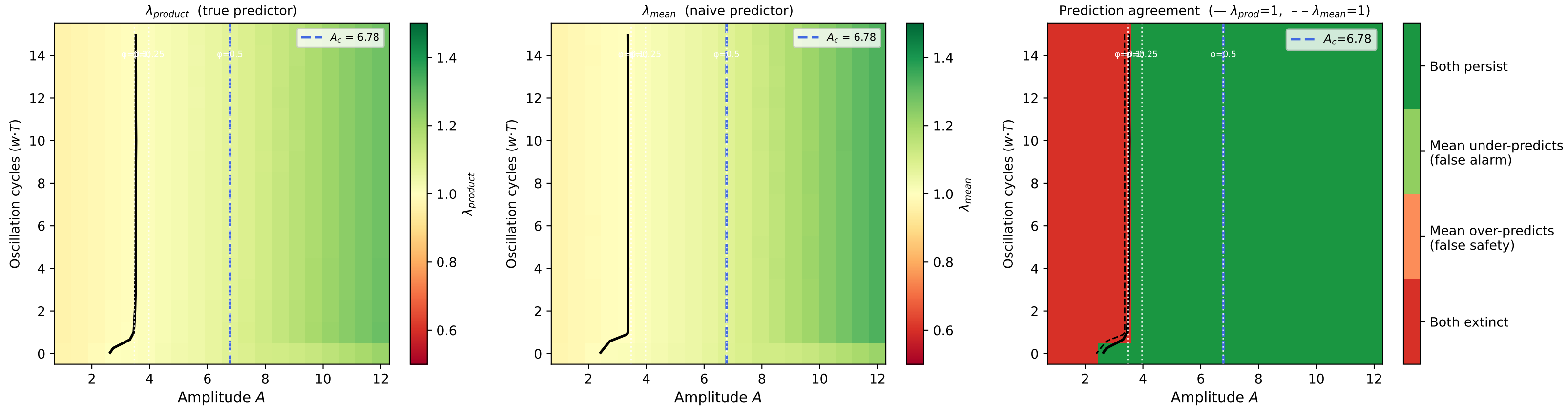
Phase Diagram: Persistence in (A, w \cdot T) Space [ n=50, T=200, c=1.0, e_0=0.001 ]
