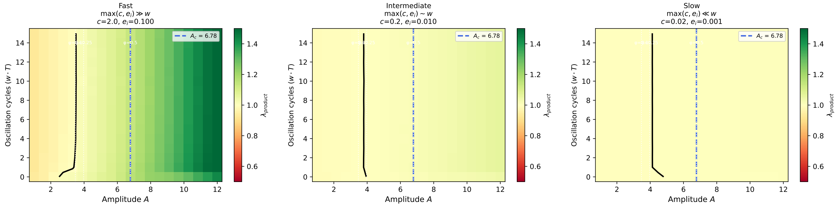
Phase Diagram for Three Demographic Regimes (coloured by \lambda_{product} , black contour = persistence threshold)
