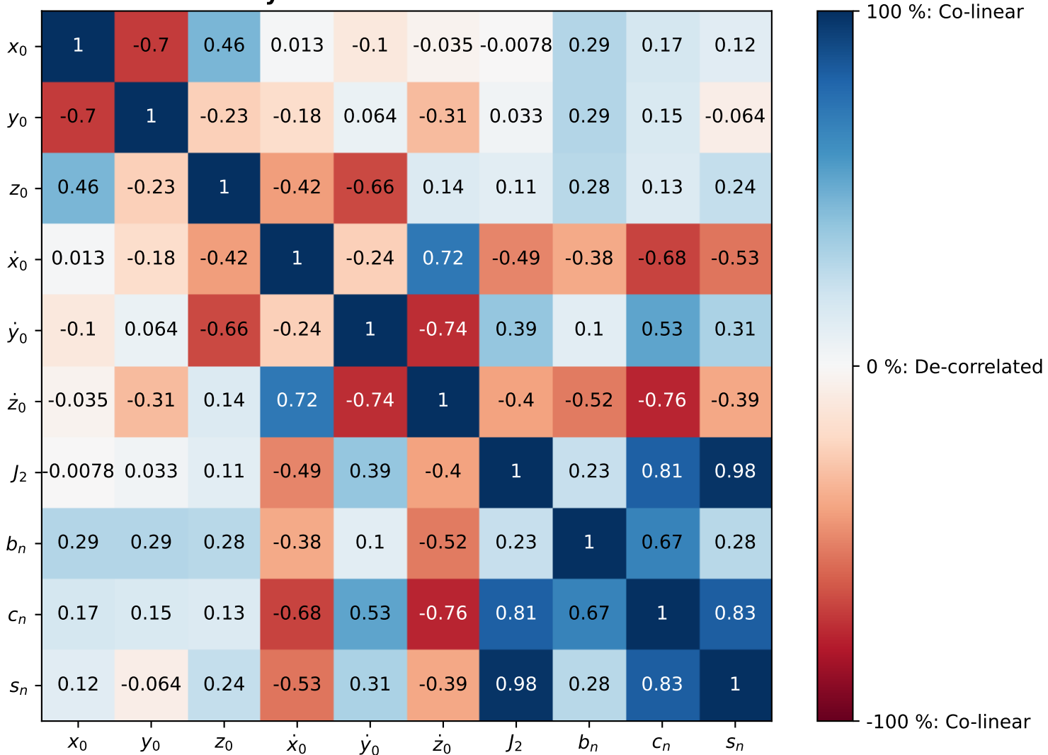
Toy-model arc correlations
