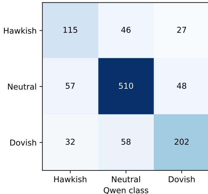
Manual vs Qwen — 3 categories
