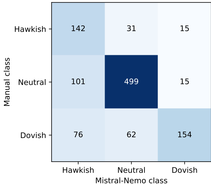
Manual vs Mistral-Nemo — 3 categories
