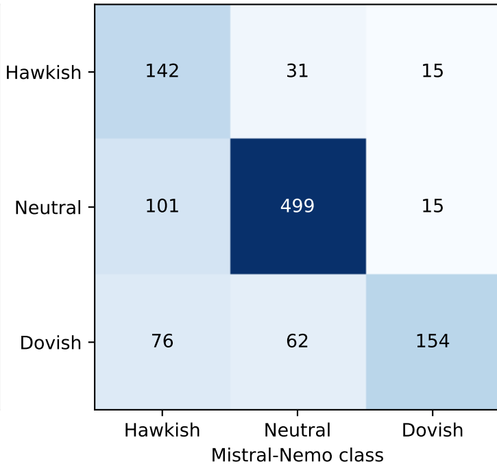
Manual vs Mistral-Nemo — 3 categories
