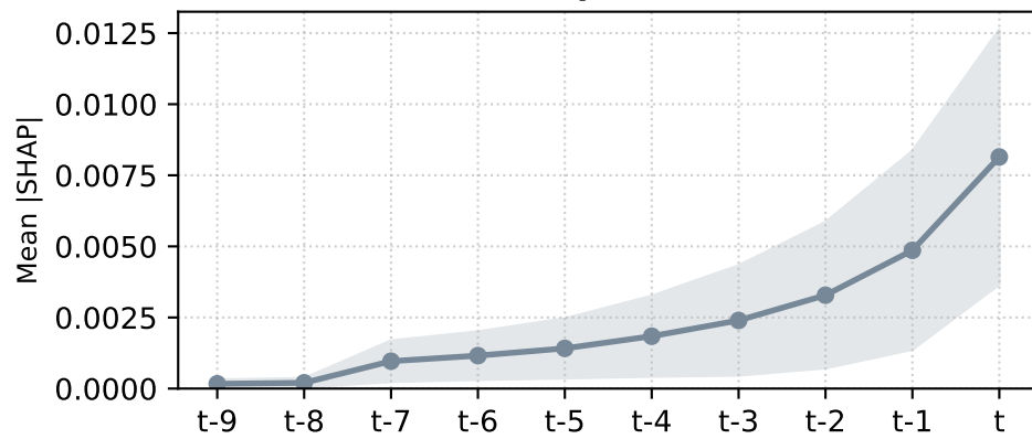
Brent
