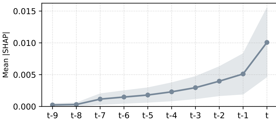
5yInflExp
