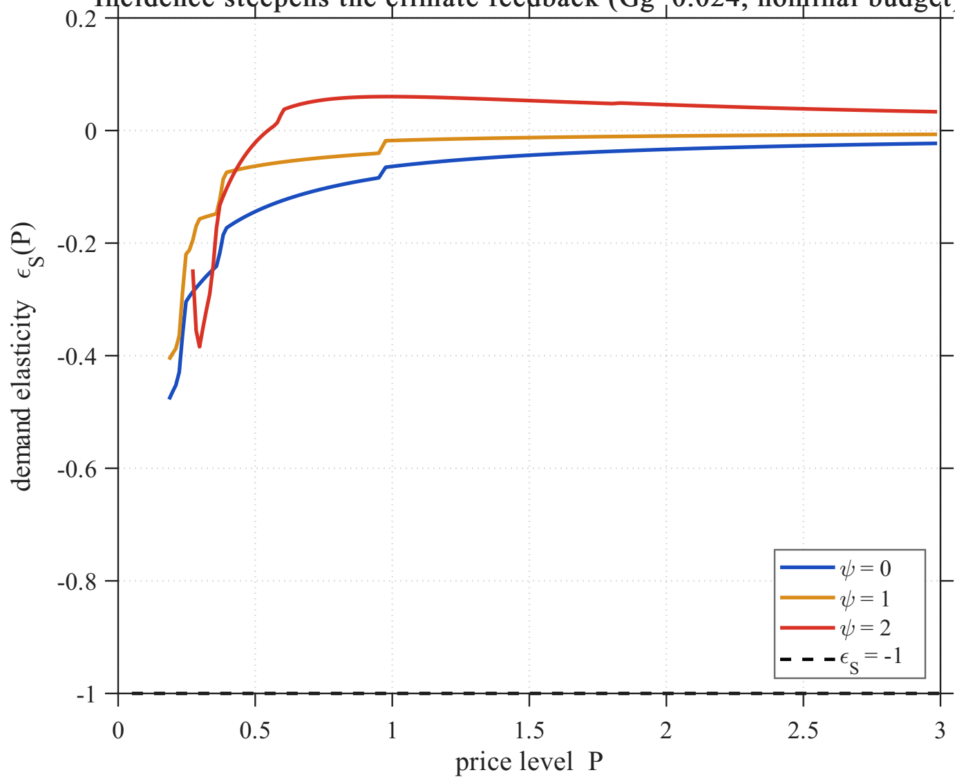
Incidence steepens the climate feedback ( Gg=0.024 , nominal budget)
