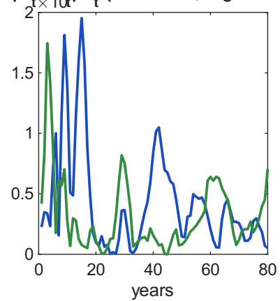
|S_t - b_t|/b_t (residuals, log scale)
