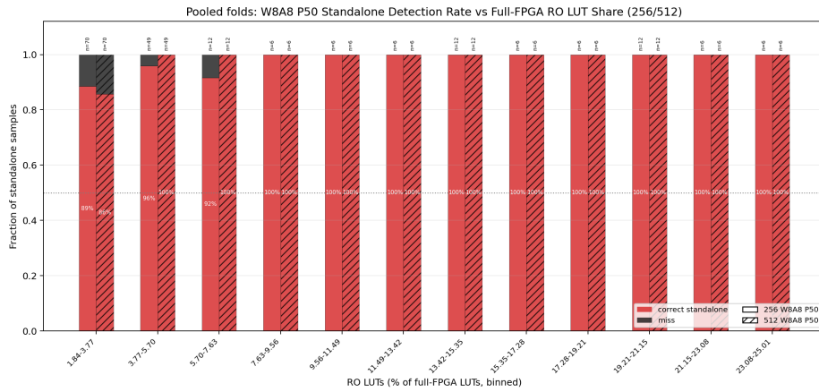
Figure 4.5: Binned standalone detection rate versus estimated RO LUT share for W8A8 P50 256×7 and 512×7 models. The smallest RO-footprint bins contain most misses, while larger evaluated RO payloads are detected reliably.
