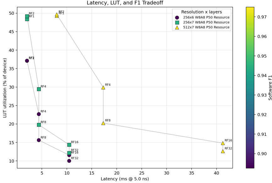
Figure 5.1: Latency, LUT utilization, and F1 tradeoff for W8A8 P50 resource-strategy candidates. Marker shapes distinguish the 256 \times 7 and 512 \times 7 reuse-factor sweeps from the base models, without manual per-layer tuning.
