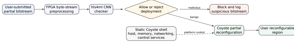
Figure 6.1: Proposed Coyote integration path. The partial-bitstream checker is placed before partial reconfiguration and decides whether the bitstream should be loaded or rejected.
