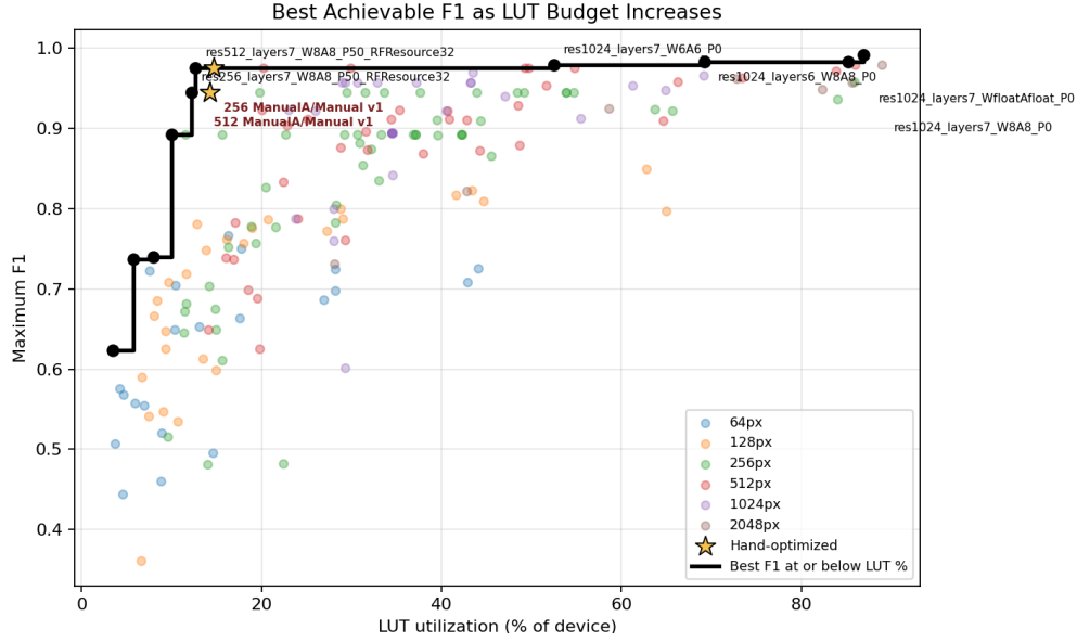
Figure 5.3: Best achievable F1 as the LUT budget increases. The black frontier shows the maximum F1 achieved by any synthesized candidate within each LUT budget. Stars indicate the manually optimized deployment candidates.
