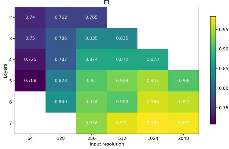
Figure 4.1: F1 score across input resolution and CNN depth. Higher resolution and deeper models improve software detection quality, but they also increase hardware cost.
