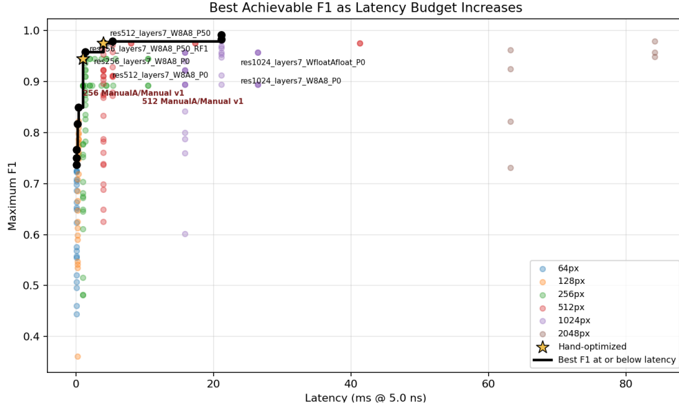
Figure 5.2: Best achievable F1 as the latency budget increases. The black frontier shows the maximum F1 achieved by any synthesized candidate within each latency budget. Stars indicate the manually optimized deployment candidates.
