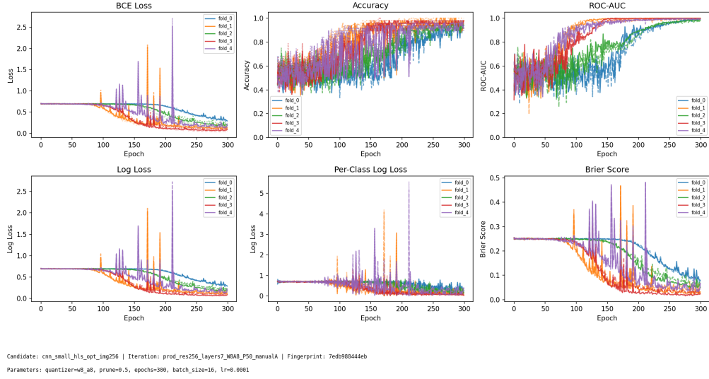
Figure 4.4: Training diagnostics for the 256×7 W8A8 P50 run. Fold 0 shows slower improvement and a higher loss trajectory than the strongest folds, motivating additional checks beyond qualitative Grad-CAM inspection.
