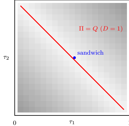
FIGURE 5. [Evidence, not proof.] The certified lower bound (1 - 2\delta)^{-1} on D(u_\tau) over the slice \tau_3 = \frac{1}{2} of the cyclic family (closed form via Theorem 7.11 and Theorem 6.13; darker = larger, from 1 (white) to \frac{3}{2} (black)). The concurrent locus in this slice is the anti-diagonal \tau_1 + \tau_2 = 1 (i.e. \Pi = Q ), where D = 1 ; the defect grows toward the facet-like corners. Certified skeleton upper bounds match this map to within 0.06 on the strip |\tau_1 + \tau_2 - 1| \leq \frac{1}{5} but degrade toward the corners (gap up to \approx 0.59 at (\frac{1}{20}, \frac{1}{20}) ), where the optimal support leaves the boundary (Remark 7.14): the map is orientation for Problems 10.1 and 10.11, not a computation of D .
