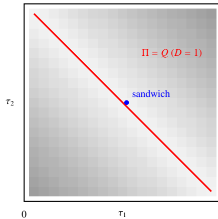
Figure 5. [Evidence, not proof.] The certified lower bound (1 - 2\delta)^{-1} on D(u_\tau) over the slice \tau_3 = \frac{1}{2} of the cyclic family (closed form via Theorem 7.11 and Theorem 6.14; darker = larger, from 1 (white) to \frac{3}{2} (black)). The concurrent locus in this slice is the anti-diagonal \tau_1 + \tau_2 = 1 (i.e. \Pi = Q ), where D = 1 ; the defect grows toward the facet-like corners. Certified skeleton upper bounds match this map to within 0.06 on the strip |\tau_1 + \tau_2 - 1| \leq \frac{1}{5} but degrade toward the corners (gap up to \approx 0.59 at (\frac{1}{20}, \frac{1}{20}) ), where the optimal support leaves the boundary (Remark 7.14): the map is orientation for Problems 10.1 and 10.12, not a computation of D .
