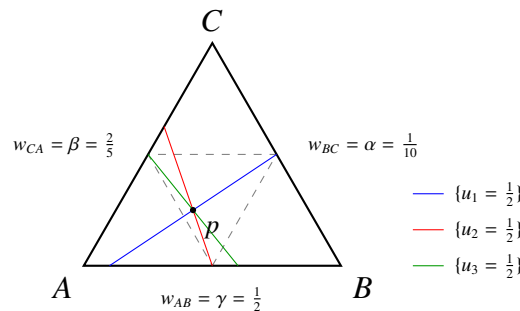
Figure 2. The weighted-perimeter witness of Theorem 6.3 at p = (\frac{9}{20}, \frac{3}{10}, \frac{1}{4}) , i.e. \tau = (\frac{5}{9}, \frac{4}{5}, \frac{1}{6}) : the three mid-level lines \{u_i = \frac{1}{2}\} concur at p , which lies in the open medial triangle (dashed), and \mu_p puts the indicated masses uniformly on the edges.
