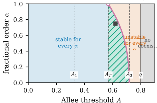
(a) Set II (generic rationals), q = 4/5
