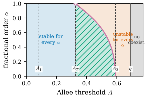
(b) Set III (irrational parameters), q \approx 0.692
