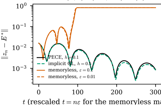
(c) Set II at (A, \alpha) = (0.62, 0.75) , \alpha^*(A) = 0.839
