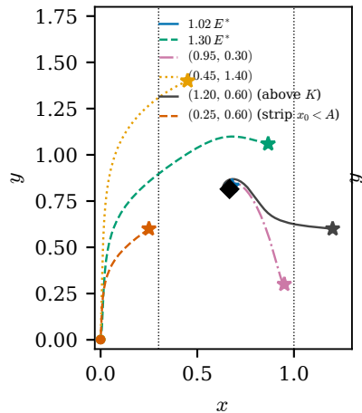
(a) \alpha = 0.9 , E^* stable
