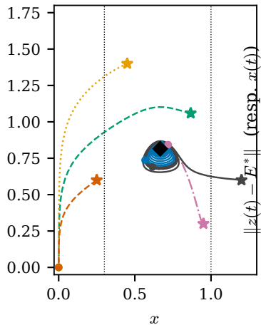
(b) \alpha = 0.99 , E^* unstable
