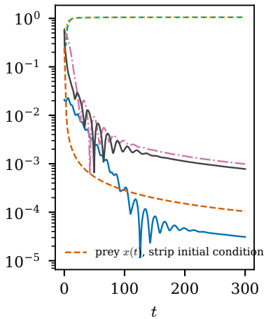
(c) \alpha = 0.9 , distance to E^*
