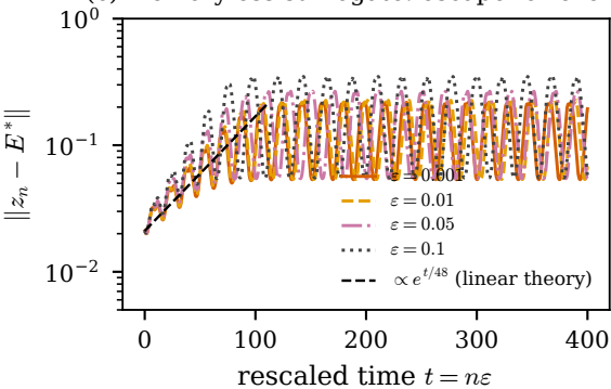
(c) memoryless surrogate: escape for every \varepsilon
