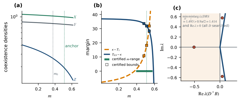
Figure 5. Certified realization W2-A. (a) Positive coexistence densities along the m -branch; at the anchor, (X, Y, Z) \approx (1, 0.786, 0.192) . (b) Classical and fractional invariant margins; marked points and the green interval are interval-certified. (c) Spectrum at the most restrictive positive diagonal found by a scale-invariant angular search. Panel (c) is numerical corroboration only: the all-diagonal statement follows from Theorem 2 and the certified invariant inequalities, not from finite search.
