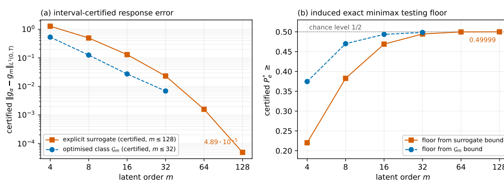
Figure 3. The certified indistinguishability floor (Theorem 2 with Table 1; certified content). (a) Interval-certified L^1 response errors: the optimized class \mathcal{G}_m to m = 32 and the explicit surrogate of Section 4.3 to m = 128 ; the latter is one admissible element, so it upper-bounds the class error. (b) The induced exact minimax floor: above 0.4996 at m = 64 and above 0.49998 at m = 128 , uniformly over all inputs with \|u\|_2 \leq 0.120 . At attainable latent orders the finite-state rival cannot be distinguished from the fractional law under this protocol by any admissible experiment.
