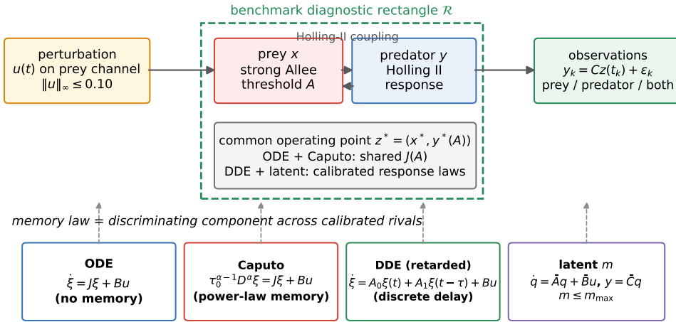
Figure 2: Setting: backbone from [15]; perturbation u(t) on the prey channel with \|u\|_\infty \leq 0.10 ; observations y_k = Cz(t_k) + \varepsilon_k on prey, predator, or both. ODE and Caputo share J(A) exactly; DDE and latent are calibrated rival response laws. Dashed rectangle: numerical benchmark diagnostic region only (not an invariant-set certificate).
