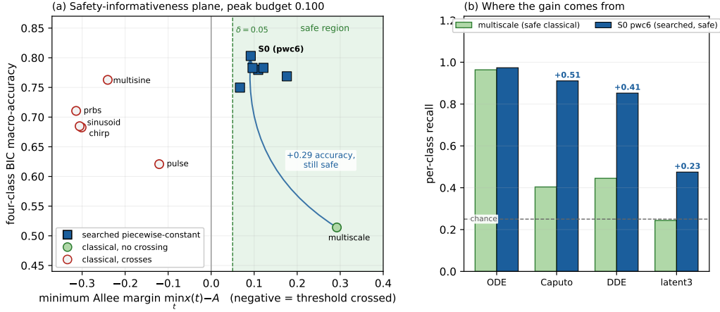
Figure 17: The safety-informativeness plane at the common peak-amplitude budget \|u\|_\infty \leq 0.100 . (a) Each point is one design: minimum Allee margin over the four candidate mechanisms against four-class BIC macro-accuracy (56 cells \times 100 replicates, identical seeds). Circles are the six classical waveform families, filled where no crossing occurs; squares are the leading designs returned by the constrained search over piecewise-constant, free-multisine and pulse-train inputs. Of the twelve designs, only multiscale and the searched PWC6 design are safe under all four mechanisms. The searched designs occupy a region of the plane that the classical families do not reach. (b) Per-class recall of the safe classical design against the leading searched design; the gain is concentrated on the Caputo and delayed mechanisms, which the safe classical design barely distinguishes from chance. The search establishes existence of such designs — Sobol sampling with local refinement over the stated families, at a single amplitude and a single \alpha — and is not a certified global optimum.
