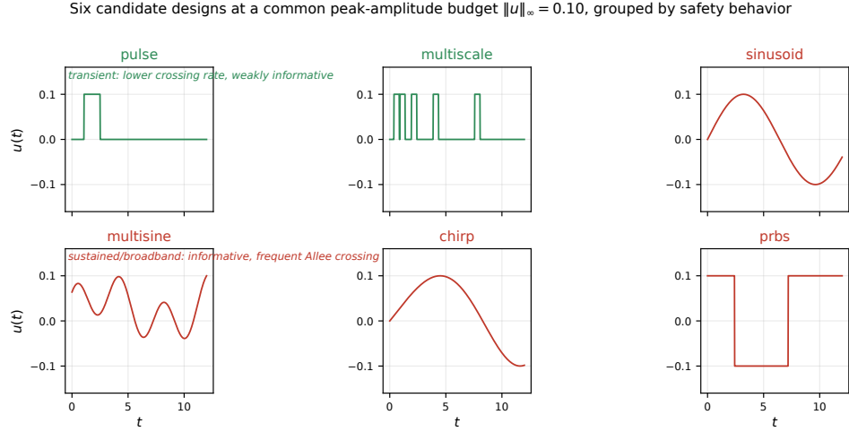
Figure 11: Six candidate perturbations at the common peak-amplitude budget. Transient and broadband designs interrogate the memory law in different ways — and behave very differently with respect to safety once the nonlinear simulations run.
