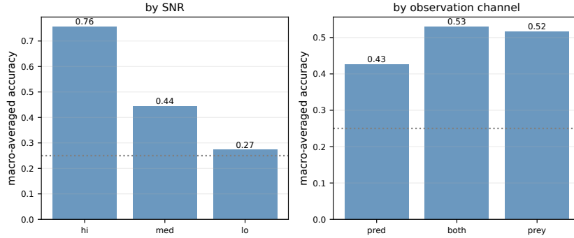
Figure 16: Accuracy stratified by SNR and observation channel. The benchmark is strongly noise-limited; observing both species gives the best average accuracy.
