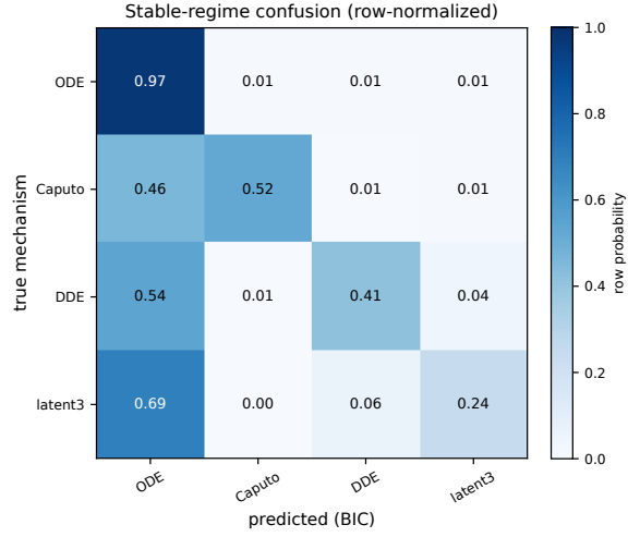
Figure 14: Row-normalized confusion matrix for the stable four-class task. Under weak excitation the simplest ODE mechanism absorbs the rest; Caputo predictions, when made, are highly precise. The finite-latent row pools data generated at latent orders m = 1 and m = 3 , both scored against the single m = 3 latent hypothesis.
