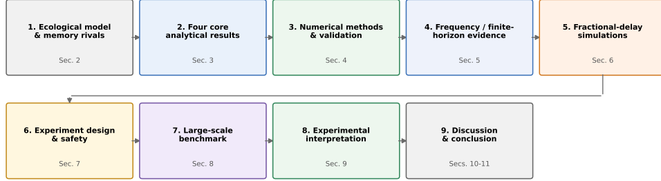
Figure 1: Structure of the paper. Sections 2–3: ecological model, rival memory laws, and the four analytical results. Sections 4–5: solver validation (Table 2) and frequency/finite-horizon evidence. Section 6: fractional-delay simulations. Sections 7–8: input design, safety, and the 1512-cell benchmark. Proofs and secondary theory: Supplementary Material.
