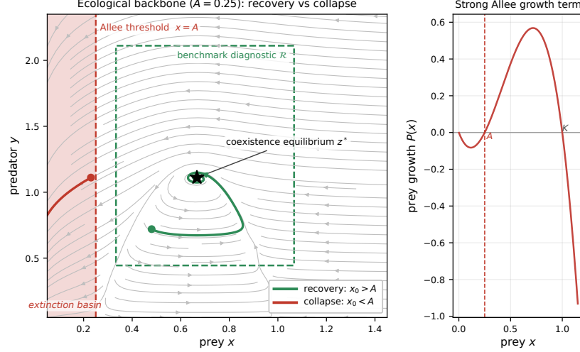
Figure 3: Safety geometry at A = 0.25 (backbone from [15]). Left: recovery for x_0 > A versus collapse for x_0 < A . Right: P(x) = rx(1 - x/K)(x/A - 1) , with sign change at x = A .
