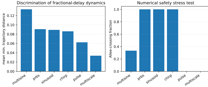
Figure 9: Input-design stress test for fractional-delay dynamics. Left: mean minimum trajectory distance from the two limiting explanations (pure Caputo and pure DDE). Right: numerical Allee-crossing fraction on the same (\alpha, \tau) grid. Broadband inputs expose the combined mechanism more strongly and are substantially less safe.
