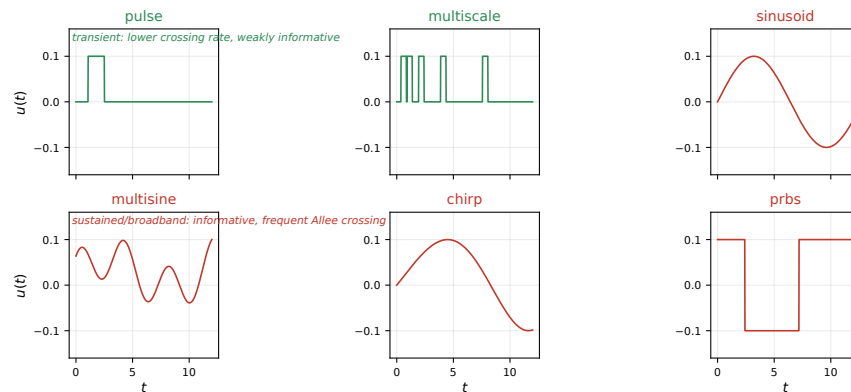
Figure 4. The six classical excitation families at the common peak budget (exposition). Broadband and sustained inputs (PRBS, multisine, chirp, sinusoid) carry the discriminating energy but drive the prey toward the threshold; the transient families are gentle and uninformative. The searched designs of Section 5.3 lie outside all six parameterizations.
