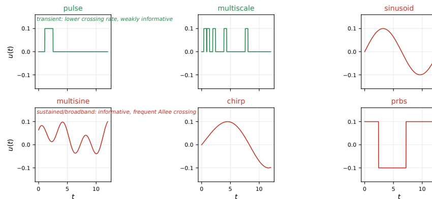
Figure 4. The six classical excitation families at the common peak budget (exposition). Broadband and sustained inputs (PRBS, multisine, chirp, sinusoid) carry the discriminating energy but drive the prey toward the threshold; the transient families are gentle and uninformative. The searched designs of Section 5.3 lie outside all six parameterizations.
