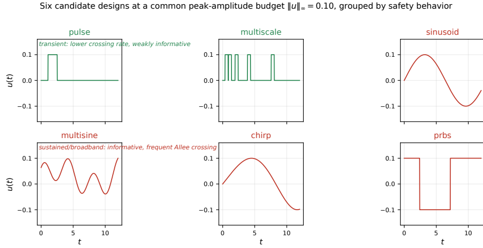
Figure 11: Six candidate perturbations at the common peak-amplitude budget. Transient and broadband designs interrogate the memory law in different ways — and behave very differently with respect to safety once the nonlinear simulations run.
