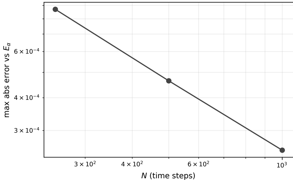
Caputo PECE convergence vs exact Mittag--Leffler solution
