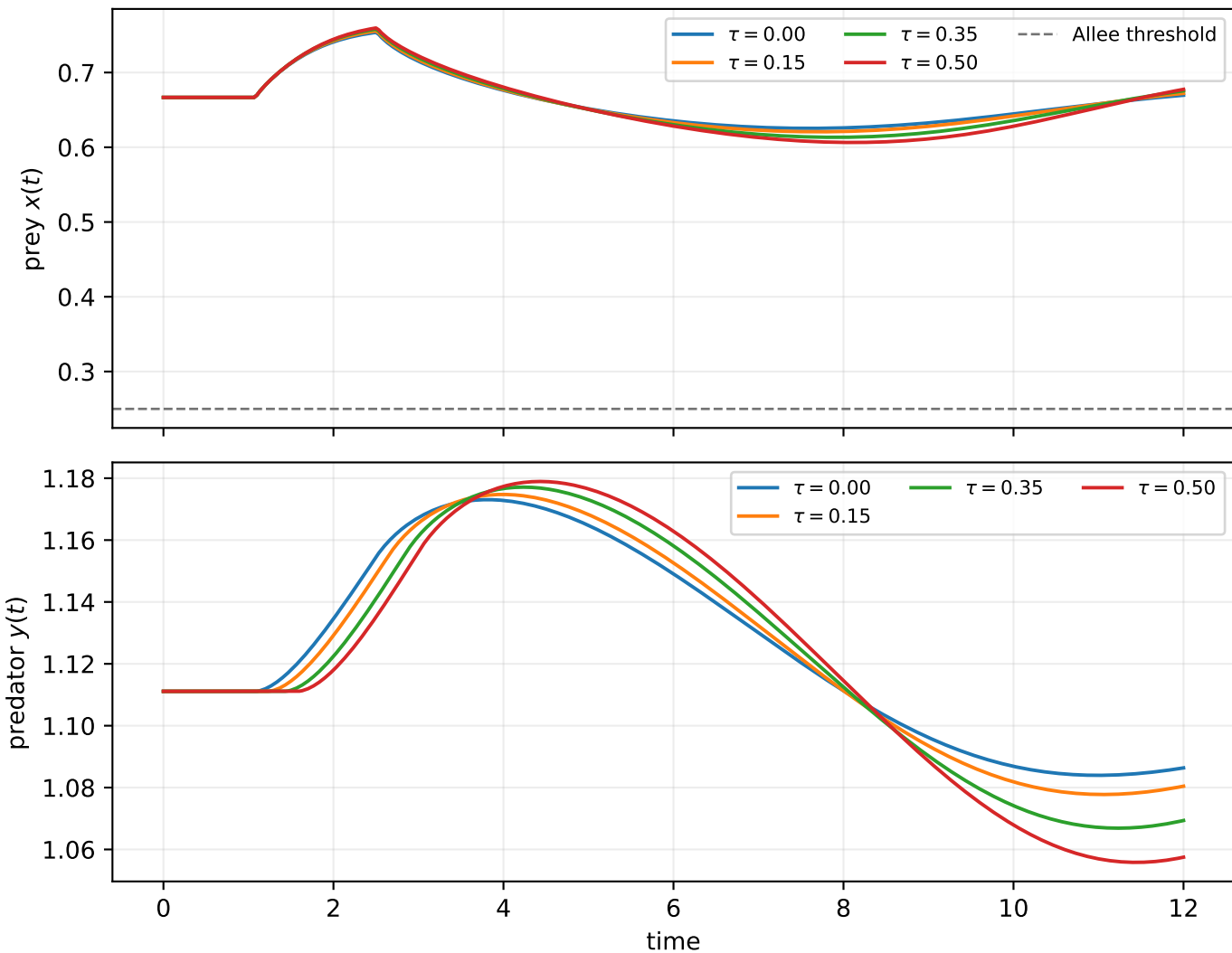
Fractional-delay response to a prey pulse ( A = 0.25 , \alpha = 0.85 )
