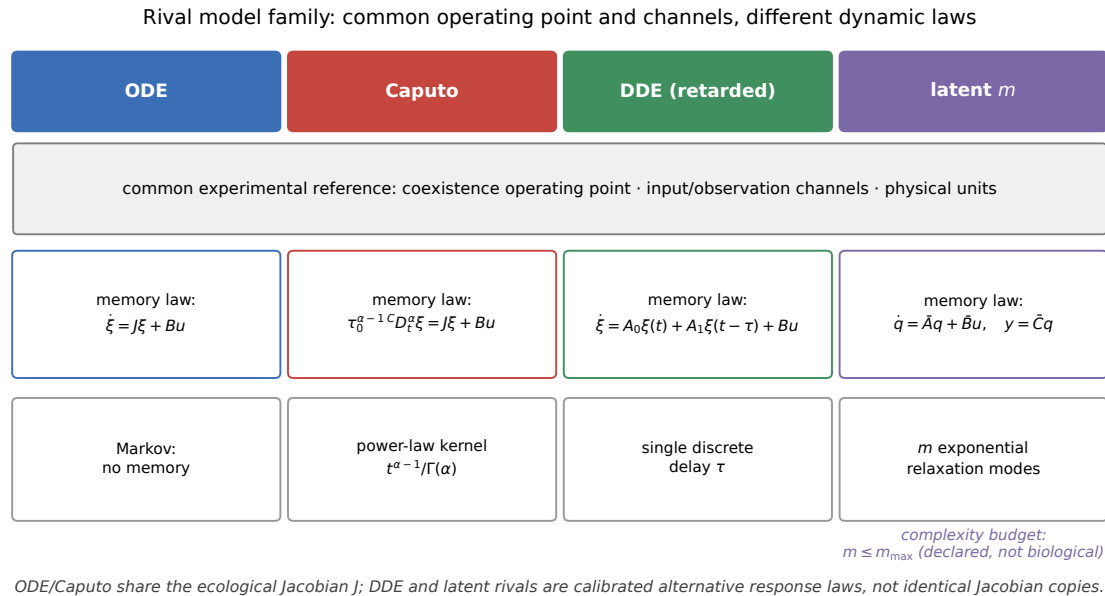
Figure S3. The rival model family. ODE and Caputo dynamics share the ecological Jacobian exactly; retarded-delay and finite-state latent rivals are alternative response laws calibrated at the same experimental operating point and compared through matched input/observation channels and units. The latent class is bounded by a declared complexity budget m \leq m_{\max} , not by a biological law.
