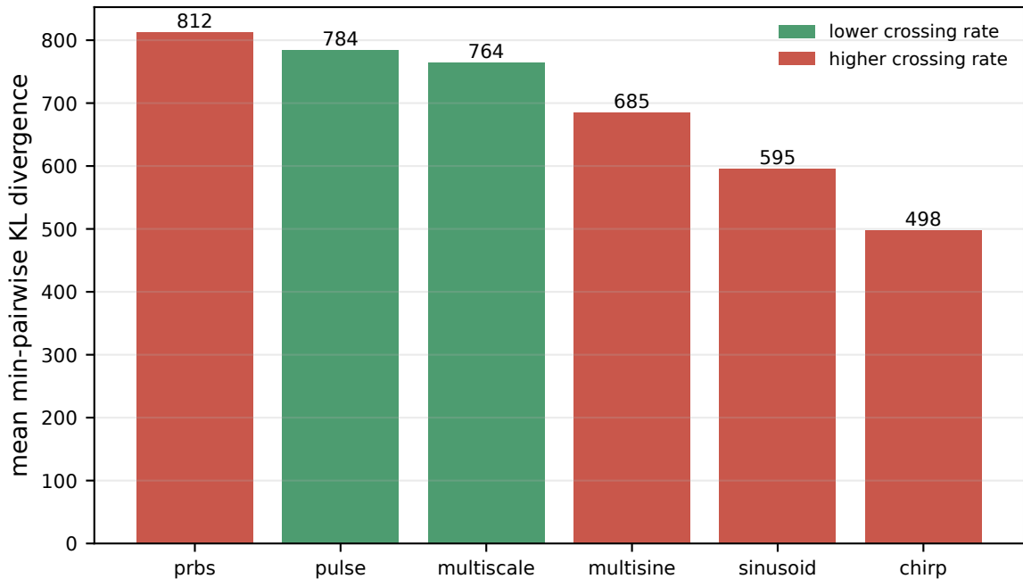
Exact linear-Gaussian design ranking (common amplitude budget)
