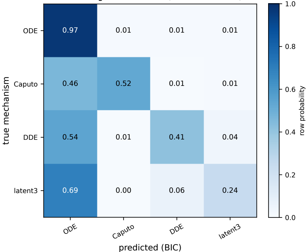
Stable-regime confusion (row-normalized)
