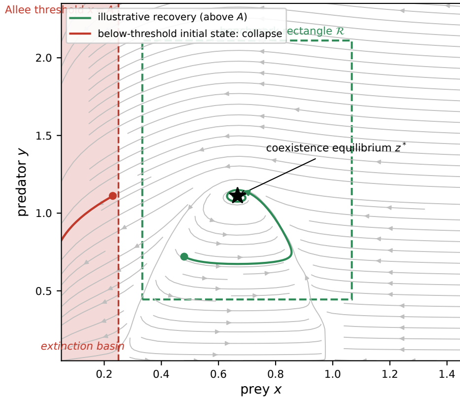
Ecological backbone ( A = 0.25 ): illustrative recovery vs collapse
