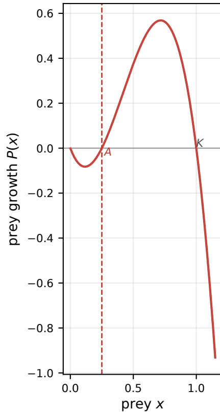
Strong Allee growth term
