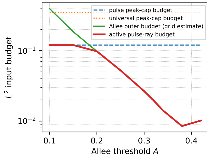
(c) Pulse-ray budget frontier \alpha = 0.85, m = 16
