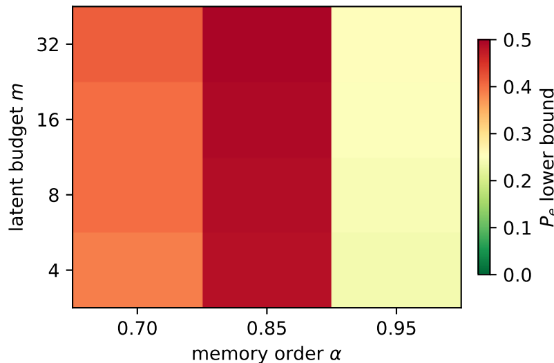
(b) Pulse-ray error lower bound A = 0.30, \sigma = 0.10
