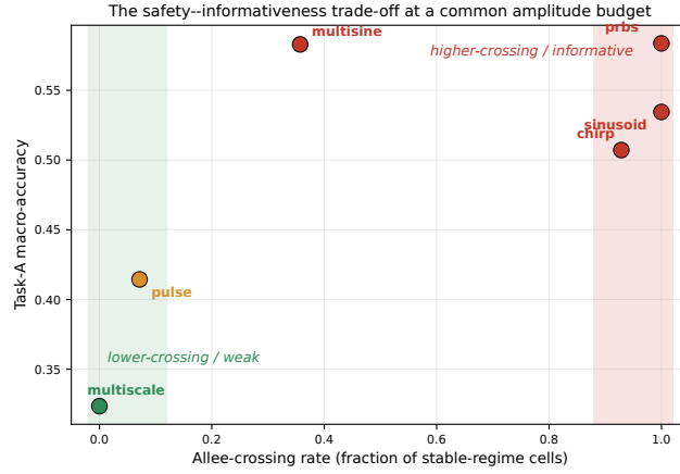
Figure 17: Headline result: the safety–informativeness trade-off at the common peak-amplitude budget. Each point is one input design, placed by its empirical Allee-crossing rate and its stable-regime macro-accuracy. Transient designs cluster in the lower-crossing/weakly-informative region; broadband designs in the high-crossing/more-informative region. No candidate in this benchmark simultaneously attains low crossing and high discrimination — which is precisely why the amplitude-capped constrained design problem is the natural next step.
