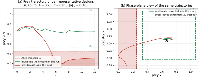
Figure 12: Safety geometry, computed with the released benchmark code for one representative stable-baseline cell ( A = 0.25 , Caputo \alpha = 0.85 , \|u\|_\infty = 0.10 ). Panel (a): the multiscale trajectory does not cross the Allee threshold in this run (minimum margin +0.369 ), whereas prbs crosses it (minimum margin -0.257 ; shaded interval marks the violation). Panel (b): the same trajectories against the benchmark diagnostic rectangle \mathcal{R} . Remaining inside this rectangle in a simulation is a numerical diagnostic, not a proof of positive invariance; Theorem 8.4 provides such a certificate only when its strict face inequalities are verified. The figure visualizes the dynamical trade-off quantified over the full benchmark in Section 10.
