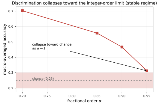
Figure 15: Model-selection accuracy versus fractional order (stable task): discrimination collapses toward the chance level of 0.25 as \alpha \rightarrow 1 , because the Caputo mechanism approaches the ODE mechanism — a direct numerical instance of the boundary degenerations flagged in Section 9.
