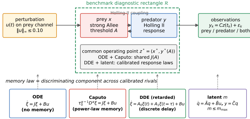
Figure 2: The object under study. A certified ecological backbone — prey with a strong Allee threshold, predator with a Holling type II response, and coexistence equilibrium z^* — receives bounded perturbations u(t) on the prey channel and is observed through prey, predator, or both channels. The ODE and Caputo mechanisms share the ecological Jacobian J(A) exactly; the retarded-DDE and finite-latent alternatives are calibrated at the same operating point and compared through matched input/observation channels and physical units, without assuming identical internal generators. The latent class carries a declared complexity budget m \leq m_{\max} . The dashed green rectangle is the benchmark diagnostic rectangle; positive invariance requires the strict inward-pointing hypotheses of Section 8 and is not implied by the rectangle definition alone.
