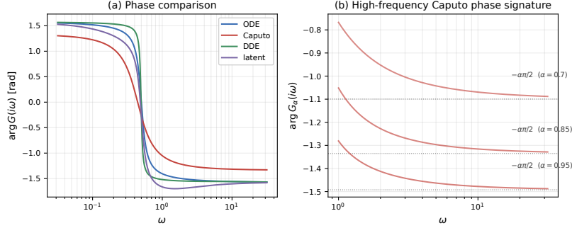
Figure 6: Phase signatures of structural separation. Panel (a): full phase comparison on the prey channel — the Caputo mechanism separates from the integer-order, delay, and latent alternatives. Panel (b): the scale-free high-frequency signature \arg G_\alpha(i\omega) \rightarrow -\alpha\pi/2 of Equation (15) for three fractional orders, converging to the dotted asymptotes. This is a collocated-channel property: cross channels ( CB = 0 ) carry a different asymptotic phase.
