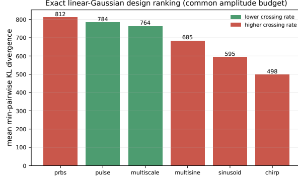
Figure 11: Exact linear-Gaussian design ranking by mean minimum pairwise KL divergence over the full factorial under the common peak-amplitude budget; state safety is not imposed in this ranking. Bars are colored by the nonlinear benchmark’s safety verdict (Figure 17): the linear optimum and the safe set disagree — the preview of the trade-off.
