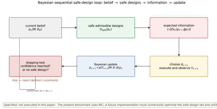
Figure 13: The Bayesian sequential safe-design loop specified in this section: current belief, posterior-conditioned safe admissible designs, expected utility via the expected-KL identity of Theorem 9.2, execution and posterior update via Theorem 9.1, and an explicit stop/continue decision. The loop is pinned down analytically and left to future work as an executed layer; the present benchmark uses BIC (Section 10).
