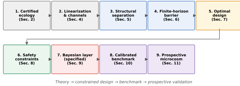
Figure 1: The paper’s pipeline. Each box names the section where the layer is developed; the main-text results are the stable-regime macro-accuracy of 0.537 against chance 0.25 and the safety–informativeness trade-off of Figure 17. A reader can reconstruct the entire argument from this figure plus the captions of Figures 2, 9, and 17.
