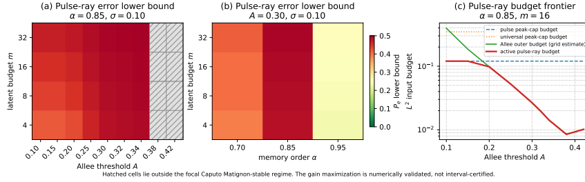
Figure 7: Protocol-restricted safe memory-discrimination atlas. Panels (a)–(b) show the Gaussian two-point lower bound for the declared positive pulse ray, using mass-valid interval enclosures of the constructive kernel error and the hierarchy-uniform Strong-Allee outer budget. Hatched cells in panel (a) lie outside the focal Caputo Matignon-stable regime and are not included in the headline stable-regime interpretation. Panel (c) shows the pulse-ray budget frontier; the Strong-Allee extremal identity of Theorem 6.10 is exact, while the displayed maximization constants and crossover are high-accuracy numerical estimates rather than interval-certified quantities. An inconclusive lower bound is never labeled discriminable.
