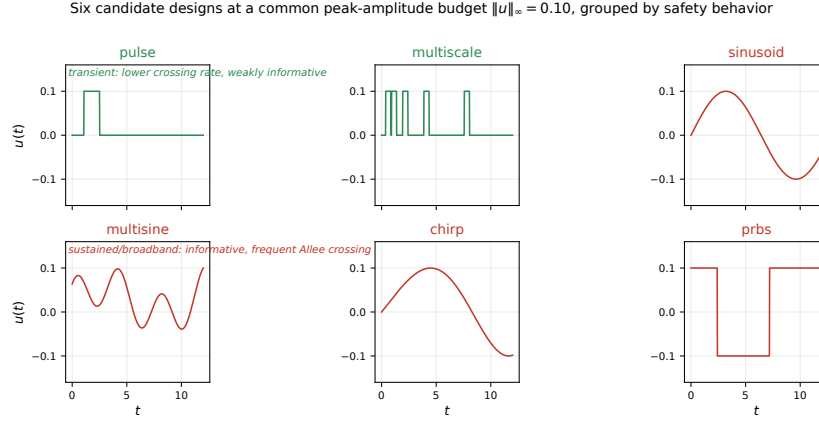
Figure 10: The six candidate input designs at the common peak-amplitude budget \|u\|_\infty = 0.10 , grouped by their benchmark safety behavior (Section 10): transient families (pulse, multiscale) have the lowest crossing rates in the benchmark but discriminate weakly; sustained/broadband families (sinusoid, multisine, chirp, prbs) are more informative yet cross the Allee threshold much more frequently.
