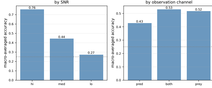
Figure 16: Accuracy stratified by SNR and observation channel (stable task): the benchmark is noise-limited (0.76 at high SNR down to 0.27 at low SNR), and both-species observation edges out the single-species channels.
