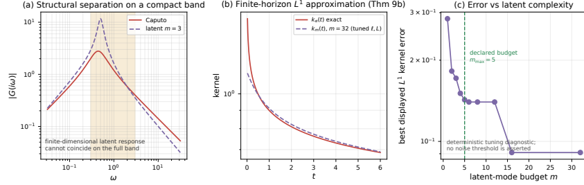
Figure 9: Exact separation versus finite-horizon approximation, in one picture. Panel (a): on a compact band the Caputo and finite-latent transfer magnitudes agree only at finitely many frequencies (Theorems 5.1–5.5); panel (b): a tuned display of the constructive exponential-sum family of Theorem 6.3 tracks the singular kernel k_\alpha in L^1(0, T) (here m = 32 ); panel (c): the deterministic best-displayed L^1 approximation error decreases as the latent-mode budget grows. The green line marks the declared modeling budget m_{\max} = 5 ; no statistical noise threshold is asserted in this panel. The theoretical fixed-noise-floor consequence is stated separately in Corollary 6.6.
