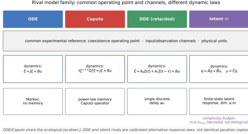
Figure 4: The rival model family. ODE and Caputo dynamics share the ecological Jacobian exactly; retarded-delay and finite-state latent rivals are alternative response laws calibrated at the same experimental operating point and compared through matched input/observation channels and units. The latent class is bounded by a declared complexity budget m \leq m_{\max} , not by a biological law.
