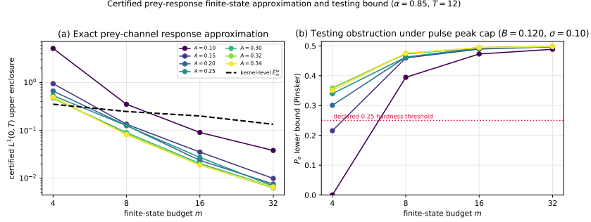
Figure 8: Certified finite-state approximation of the exact fractional prey response. Panel (a): outward-rounded L^1(0, T) enclosures \hat{E}_m^{state} across the Matignon-stable \alpha = 0.85 cells, compared with the earlier kernel-level enclosures. Panel (b): the corresponding Pinsker testing lower bound for the declared pulse under the physical peak cap \|u\|_\infty \leq 0.10 ( B \leq 0.120 ) and \sigma = 0.10 . The figure intentionally does not use the broad mass-only Strong-Allee witness; see Remark 6.15.
