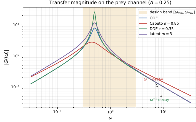
Figure 5: Transfer magnitude |G(i\omega)| on the prey channel for the four memory mechanisms at A = 0.25 . The shaded region is the design band where the optimal inputs of Section 7 place their energy; inside it the Caputo curve already separates from its rivals, with the \omega^{-\alpha} (Caputo) versus \omega^{-1} (DDE) asymptotics taking over at higher frequency.
