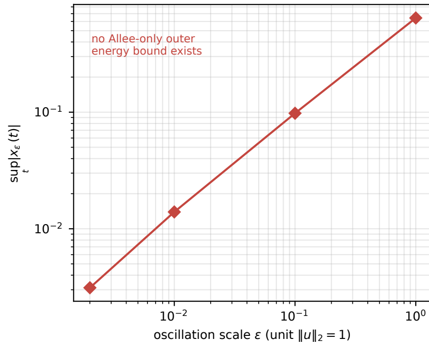
(b) Null direction: prey excursion \rightarrow 0 as \varepsilon \rightarrow 0
