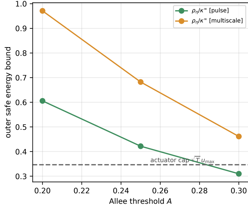
(c) Outer bound: coercive class vs actuator cap
