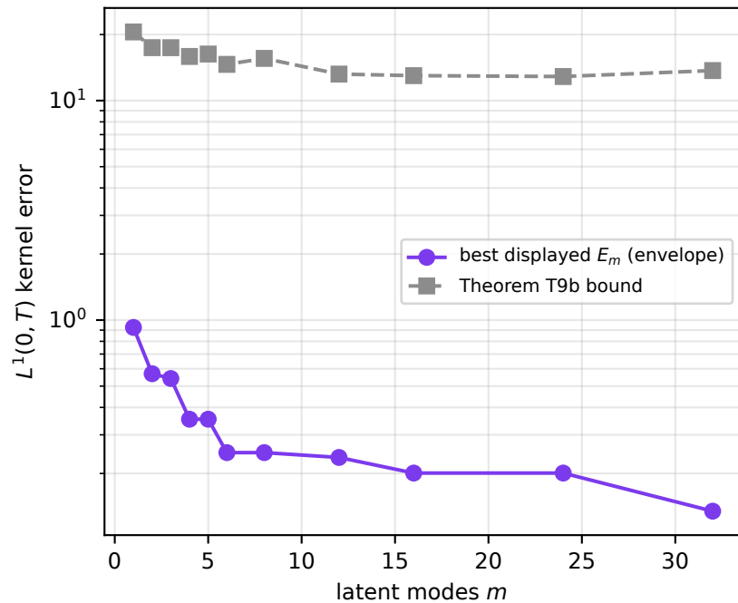
(a) Latent approximation error E_m(\alpha, T)
