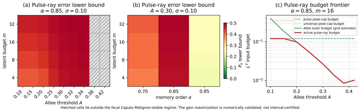
Figure 8. Protocol-restricted discrimination atlas over (\alpha, A, m) : lower bound on the model-selection error under the declared pulse protocol. The bound increases with latent budget m and toward weakly separated regimes; hatched cells violate the Matignon condition \alpha < \alpha^*(A) and are excluded from stable-regime conclusions.
