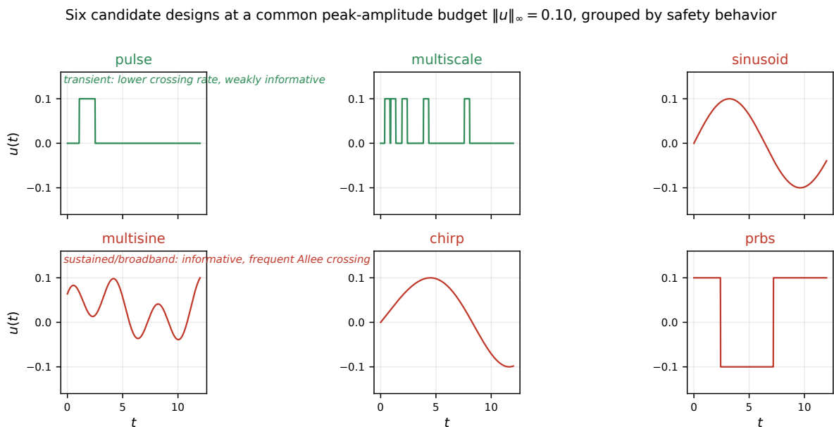
Figure 13. Six candidate perturbations at the common peak-amplitude budget. Transient and broadband designs interrogate the memory law in different ways — and behave very differently with respect to safety once the nonlinear simulations run.
