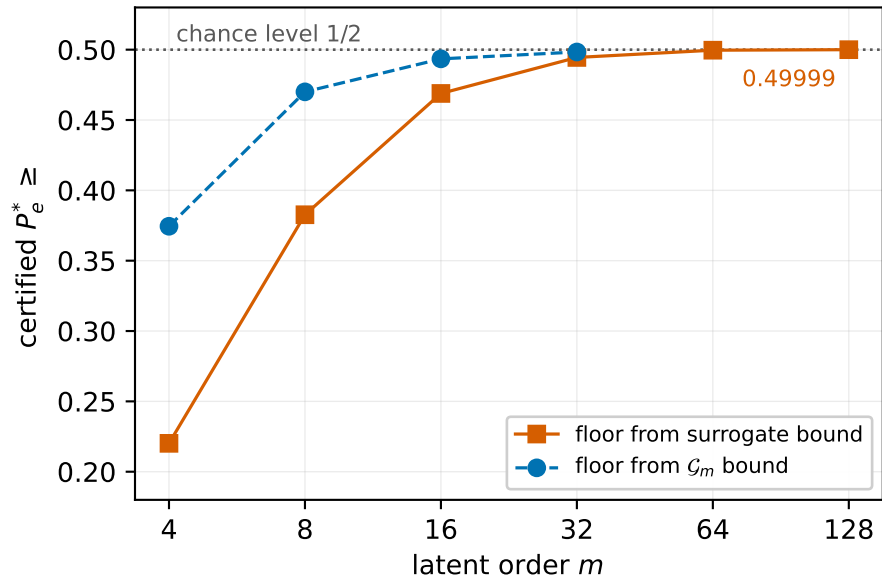
(b) induced exact minimax testing floor
