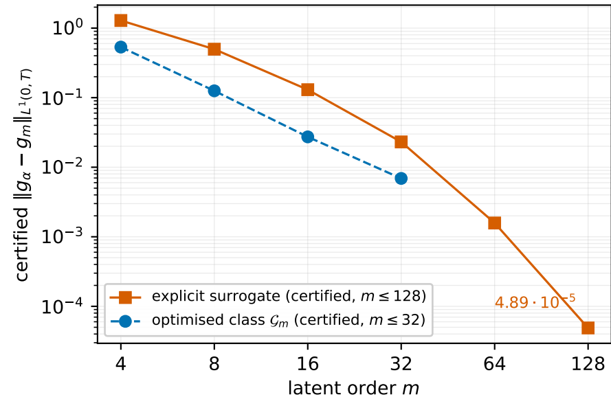
(a) interval-certified response error
