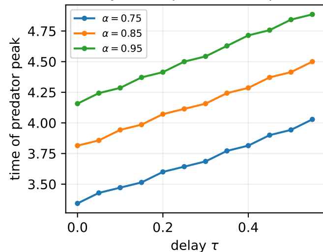
Delay shifts predator response
