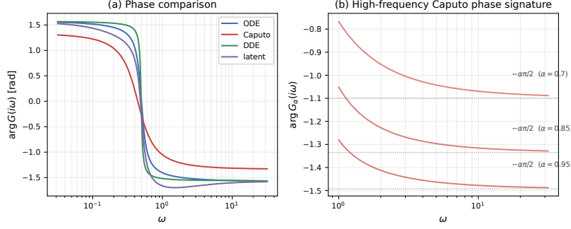
Figure S5: Phase signatures of structural separation. Panel (a): full phase comparison on the prey channel — the Caputo mechanism separates from the integer-order, delay, and latent alternatives. Panel (b): the scale-free high-frequency signature \arg G_\alpha(i\omega) \rightarrow -\alpha\pi/2 of Equation (S15) for three fractional orders, converging to the dotted asymptotes. This is a collocated-channel property: cross channels ( CB = 0 ) carry a different asymptotic phase.
