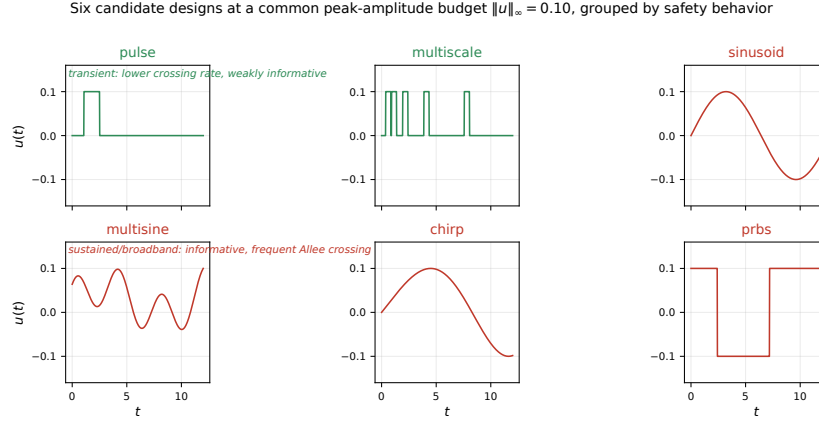
Figure S9: The six candidate input designs at the common peak-amplitude budget \|u\|_\infty = 0.10 , grouped by their benchmark safety behavior (the main-paper benchmark): transient families (pulse, multiscale) have the lowest crossing rates in the benchmark but discriminate weakly; sustained/broadband families (sinusoid, multisine, chirp, prbs) are more informative yet cross the Allee threshold much more frequently.
