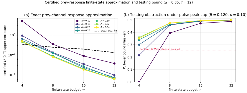
Figure S7: Certified finite-state approximation of the exact fractional prey response. Panel (a): outward-rounded L^1(0, T) enclosures \hat{E}_m^{\text{state}} across the Matignon-stable \alpha = 0.85 cells, compared with the earlier kernel-level enclosures. Panel (b): the corresponding Pinsker testing lower bound for the declared pulse under the physical peak cap \|u\|_\infty \leq 0.10 ( B \leq 0.120 ) and \sigma = 0.10 . The figure intentionally does not use the broad mass-only Strong-Allee witness; see Remark S5.15.
