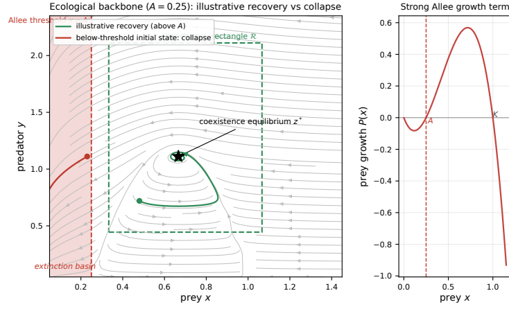
Figure S2: Ecological backbone at the benchmark baseline A = 0.25 (stable regime, integer-order skeleton). Left: an illustrative phase portrait with the rigorously established Allee threshold x = A and extinction strip, the benchmark diagnostic rectangle \mathcal{R} around z^* , and two numerically integrated trajectories: recovery from above threshold and collapse from below A . The plotted rectangle and trajectories are visual diagnostics, not an invariant-set certificate; invariance requires Theorem S7.4's strict face conditions. Right: the strong-Allee growth term P(x) , whose negative branch below A explains why safety cannot be an afterthought.
