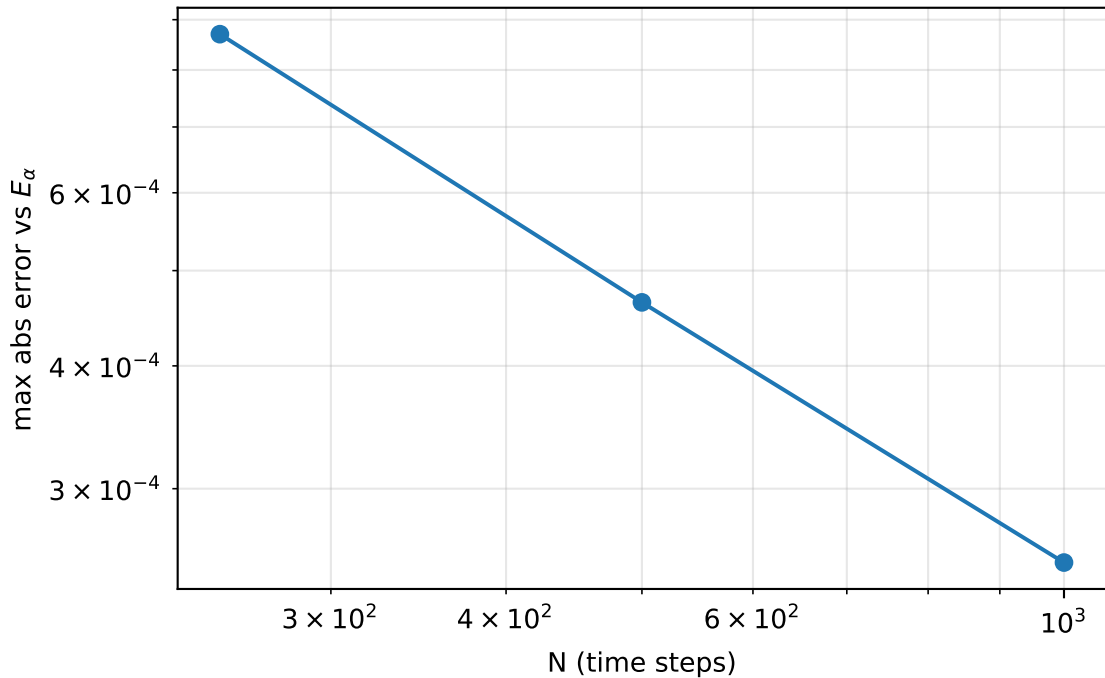
Caputo PECE convergence vs Mittag--Leffler
