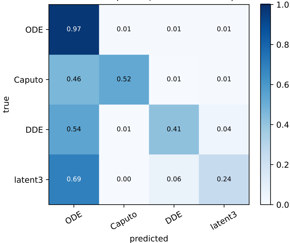
Confusion (stable, row-normalized)
