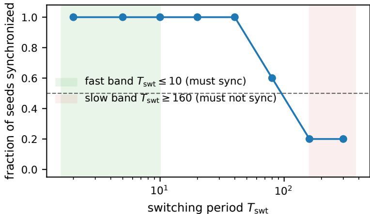
G0B calibrated demonstration ( \sigma_{12} = 1.5 , N = 40 ): PASS confirmatory; 5/5 seeds per cell, zero failures
