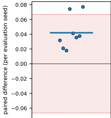
G1-weak: \gamma_{\text{arm}} - \gamma_{\text{static}} confirmatory: INCONCLUSIVE (TIE) 8/8 positive, p = 0.0078 ; mean < band
