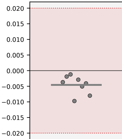
G1-strict: \gamma_{\text{arm}} - \max(\gamma_{\text{avg}}, \gamma_{\text{best}}) DIAGNOSTIC (NOT_INTERPRETABLE) 8/8 negative
