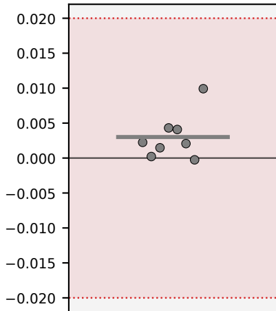
G2: \gamma_{\text{ordered}} - \text{med}(\gamma_{\text{perm}}) DIAGNOSTIC (NOT_INTERPRETABLE) p = 0.070 , not significant
