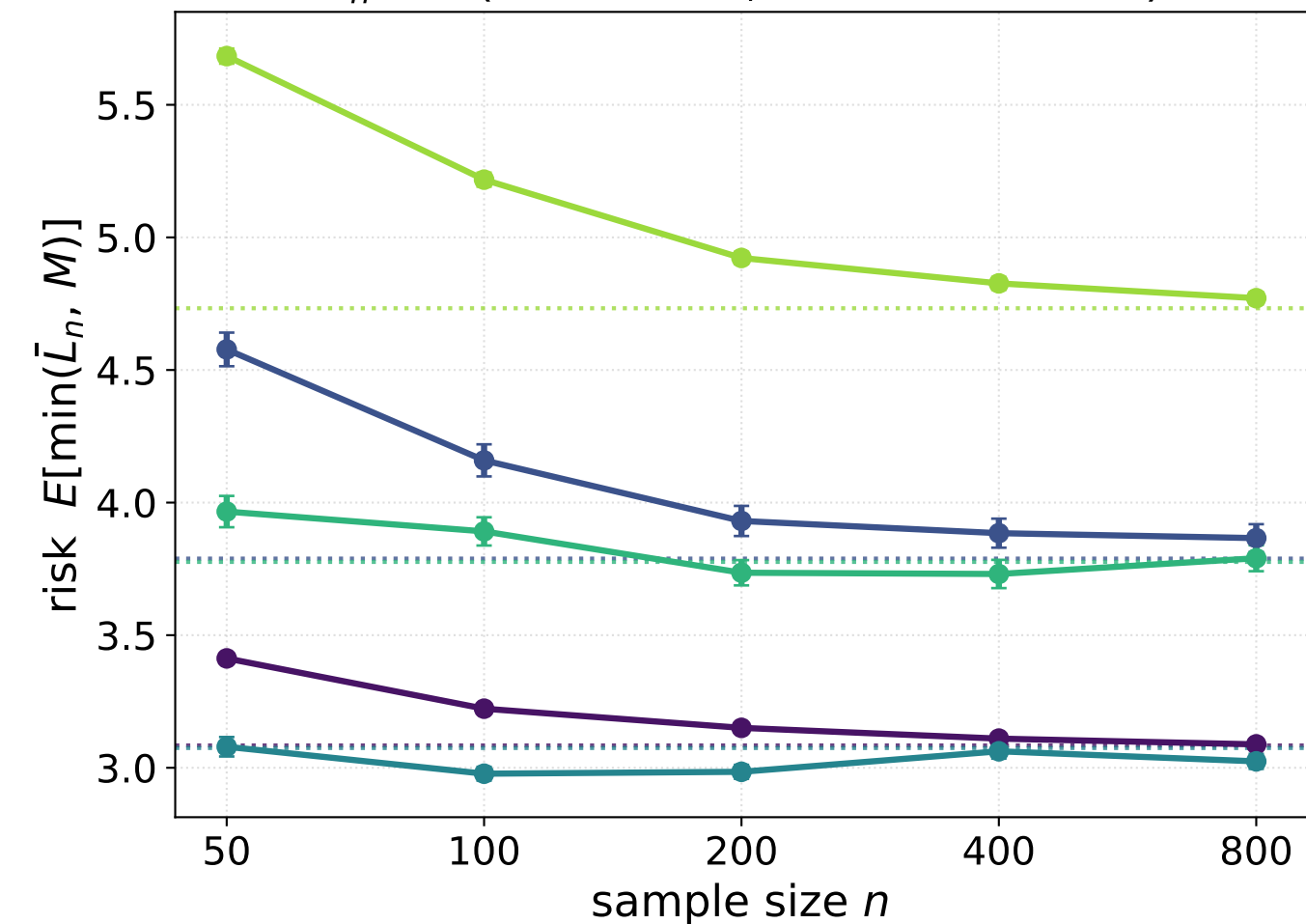
R_n \rightarrow R (Theorem 1; dotted = limit R )
