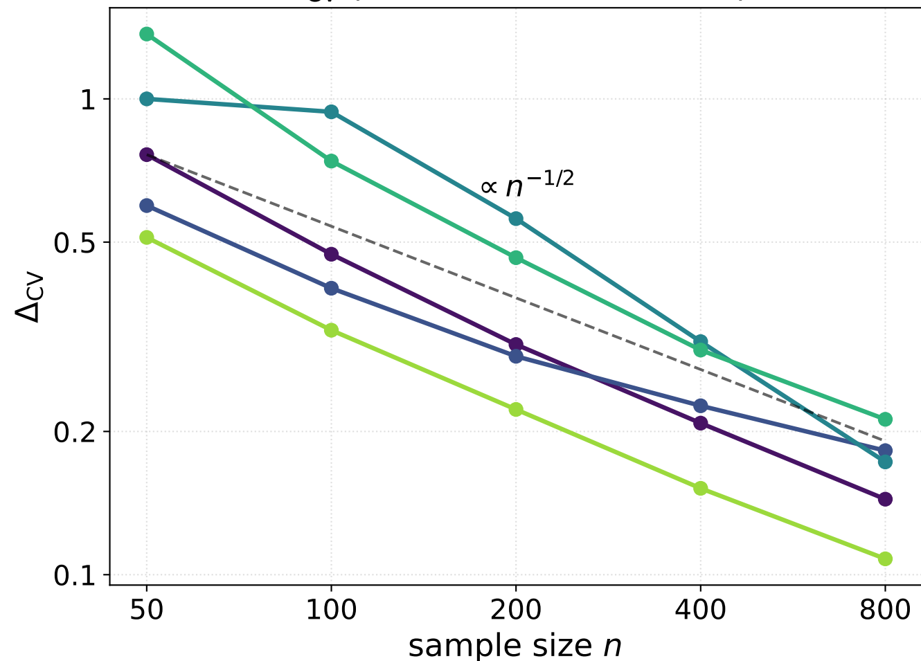
\Delta_{\text{CV}} (Lemma 4: CV \approx SURE)
