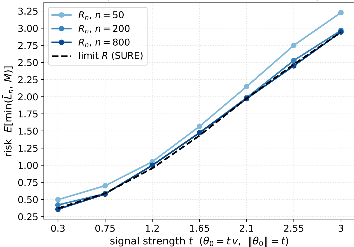
Convergence of the risk function (Linear / Ridge)
