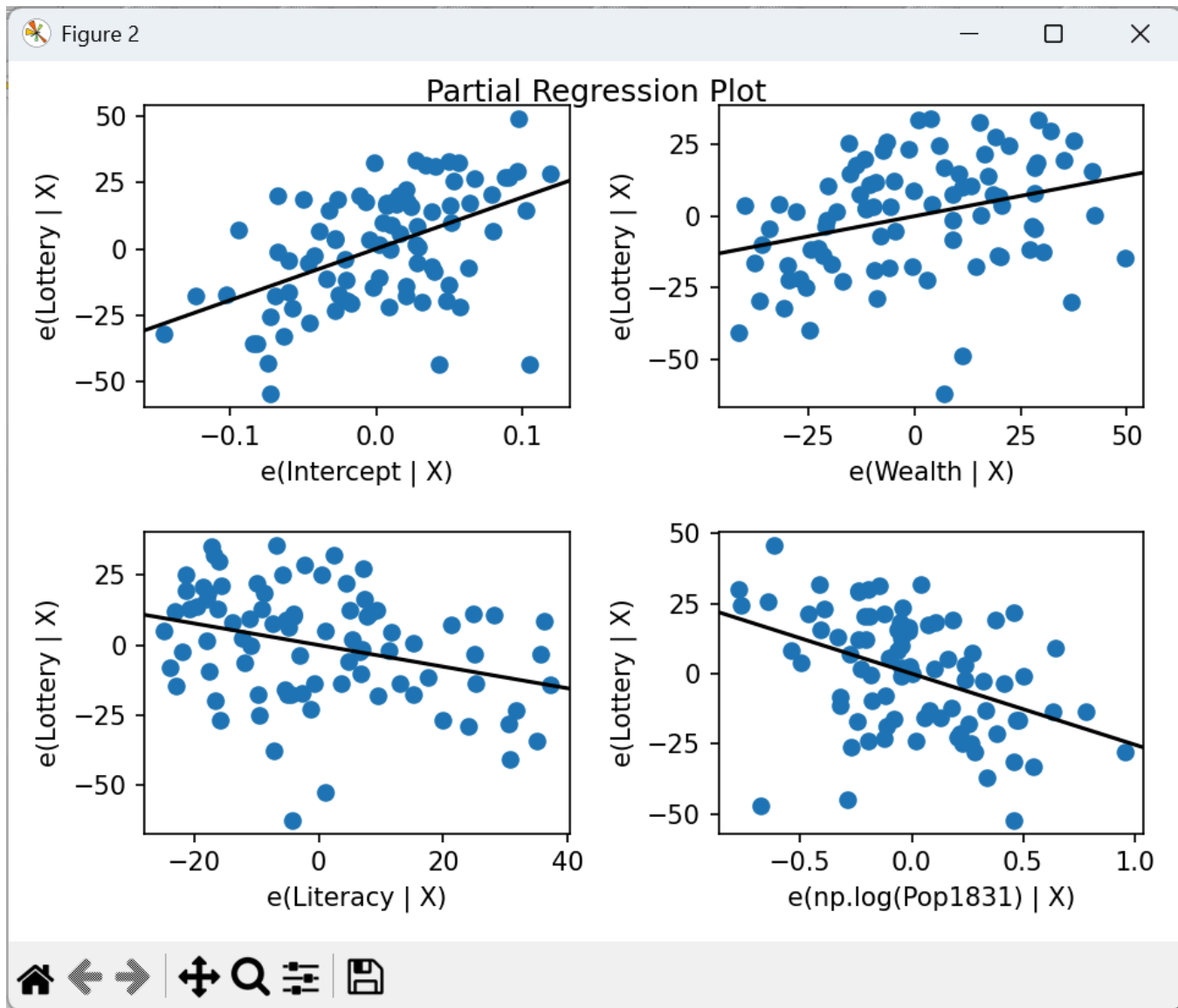
Lottery and Population
