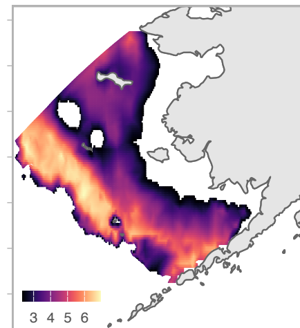
(c) log(predicted density) G. chalcogrammus (a)
