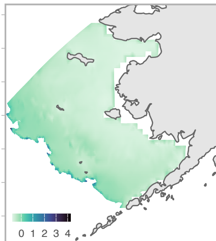
(b) Diffused depth G. chalcogrammus (a)
