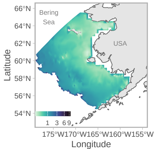
(a) log(depth)
